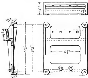
Figs. 2641-2643. Air Pump Bracket Atlantic (4-1-2) Locomotive. P. R. R.
